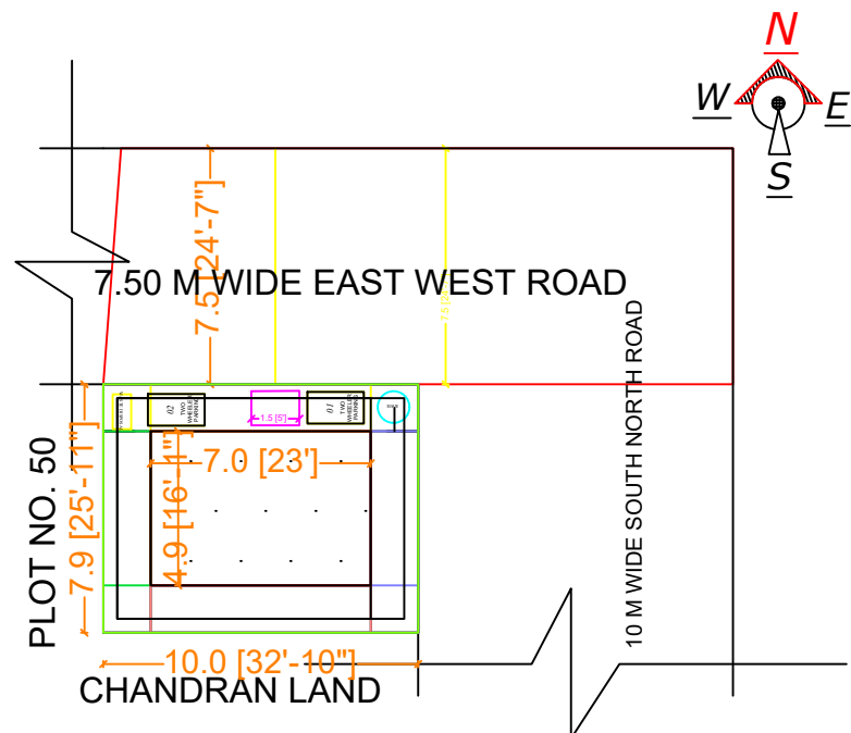
SITE PLAN
