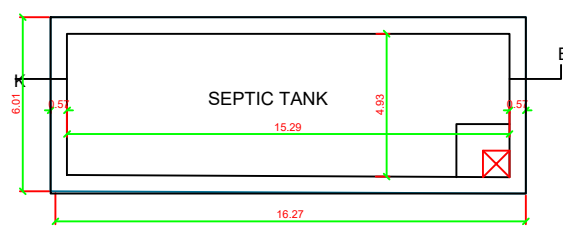
PLAN OF SEPTIC TANK SEPTIC TANK
