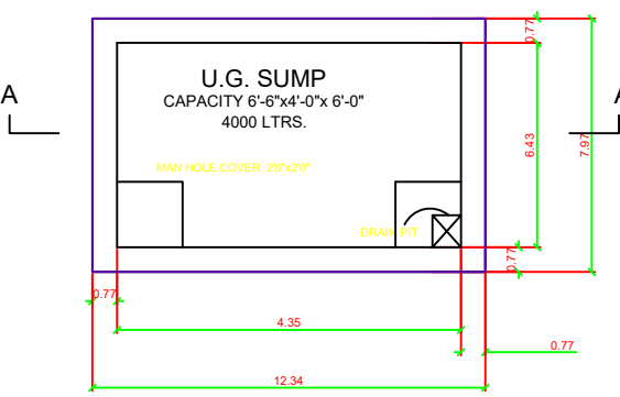
SUMP DETAIL
