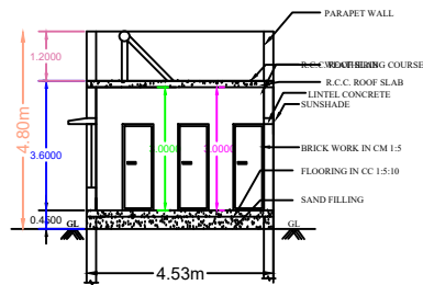
SECTION AB
