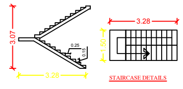
STAIRCASE DETAILS
