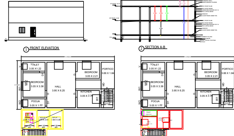
PARTIAL FIRST FLOOR & PARTIAL FIRST FLOOR PLAN
