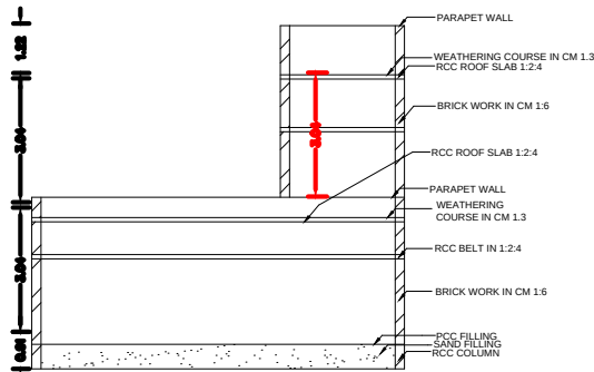
SECTION ON-AA&BB
