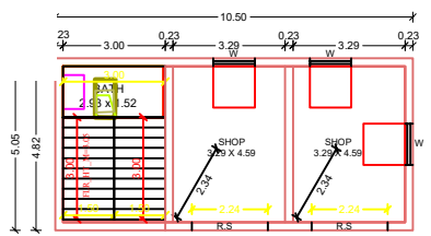
PRO.GROUND FLOOR PLAN
