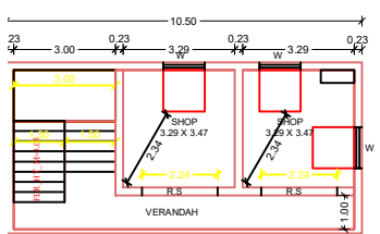
PRO.FIRST FLOOR PLAN
