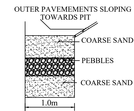
RAIN WATER PERCOLATION BED
