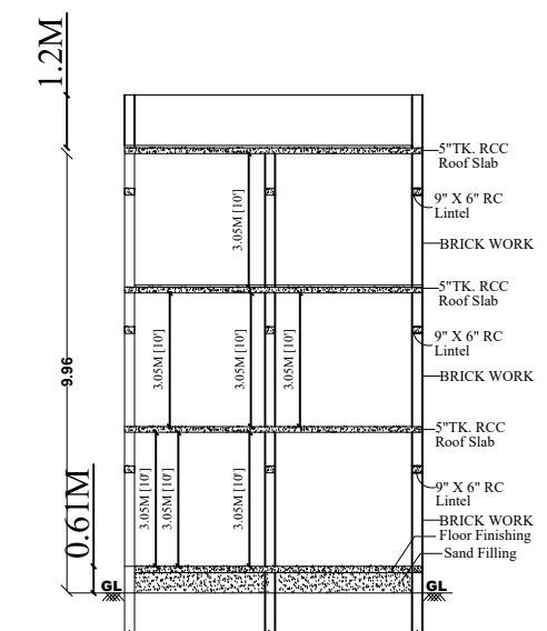
SECTION ON "SR"
