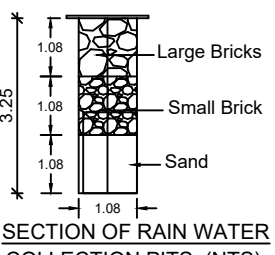
SECTION OF RAIN WATER COLLECTION PITS (NTS)
