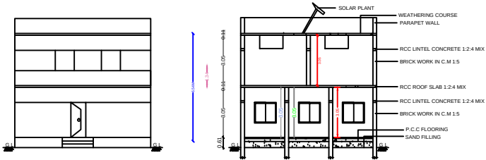
FRONT ELEVATION
