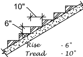
STAIR DETAIL
