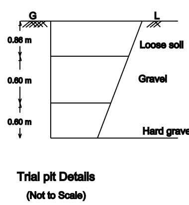
Trial pit Details (Not to Scale)
