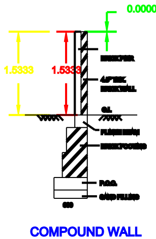
COMPOUND WALL
