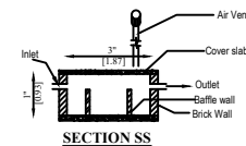
SECTION SS
