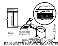
RAIN WATER HARVESTING SYSTEM
