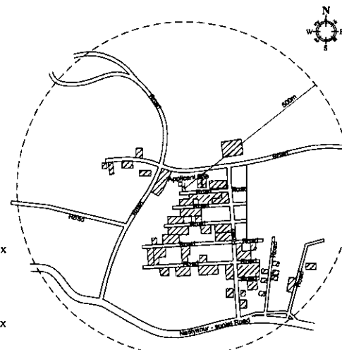
TOPO PLAN SCALE 1:5000
