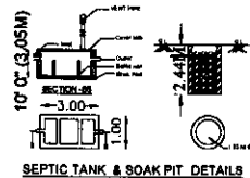
SEPTIC TANK & SOAK PIT DETAILS
