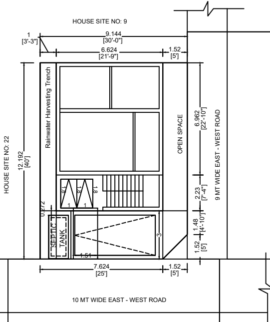
SITE CUM GROUND FLOOR PLAN
