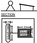
PLAN SOLAR SYSTEM
