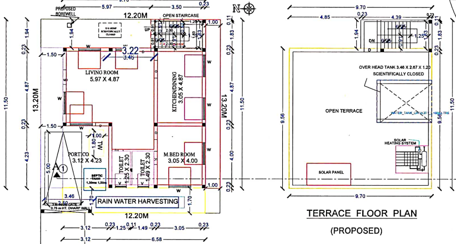
SITE/GROUND FLOOR PLAN (PROPOSED)
