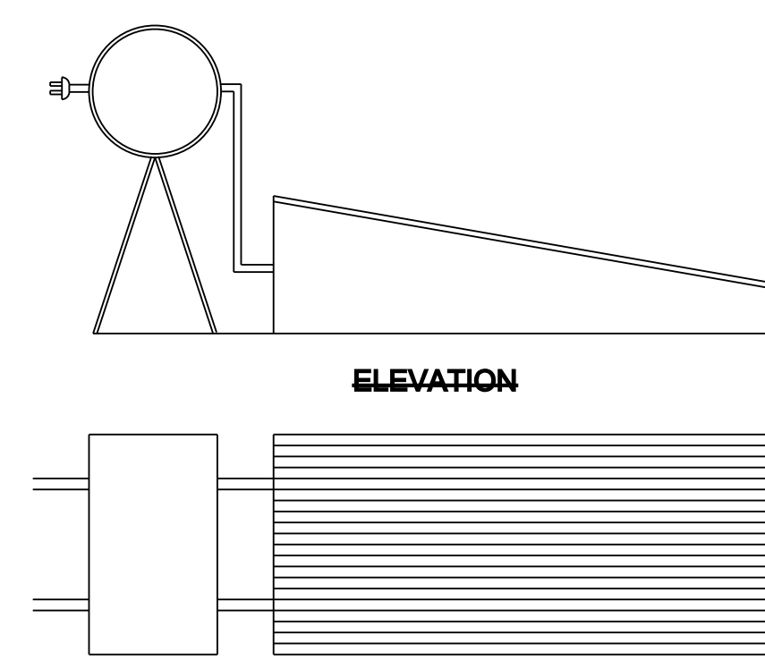
SOLAR PANEL PLAN NOT TO SCALE
