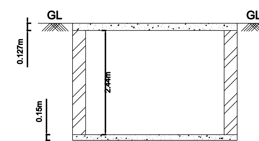
SECTION-DD
