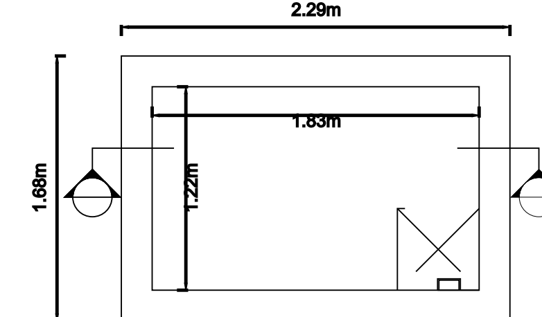
UG SUMP PLAN
