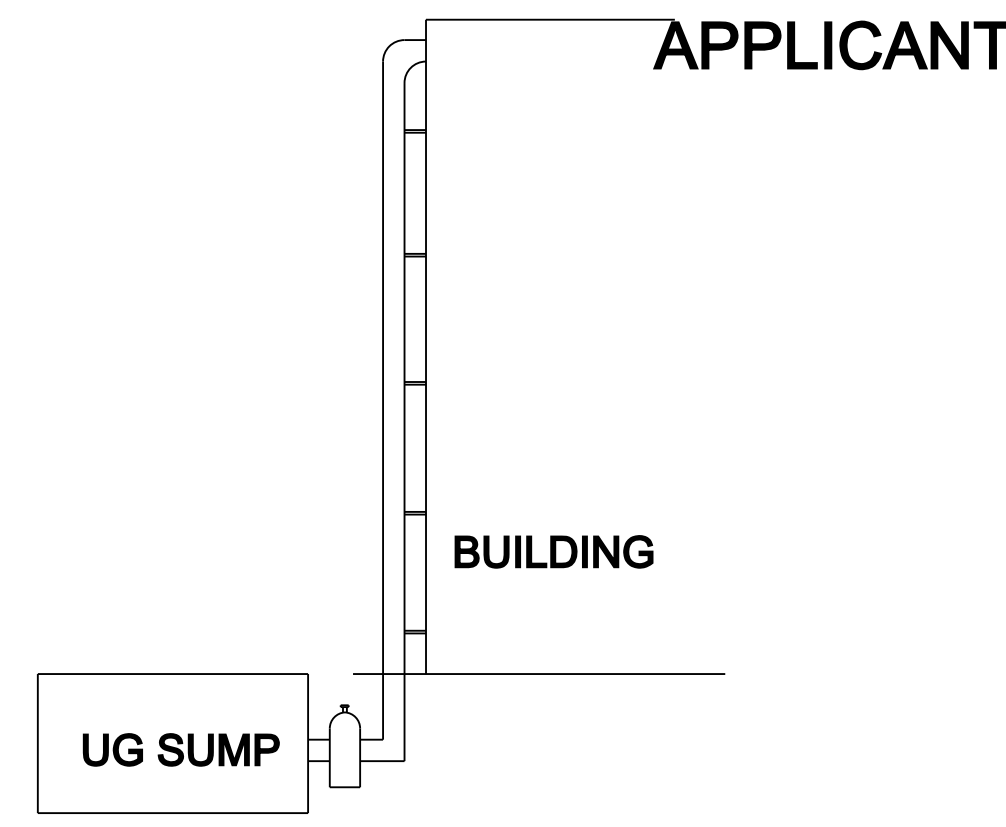
RAIN WATER HARVESTING NOT TO SCALE
