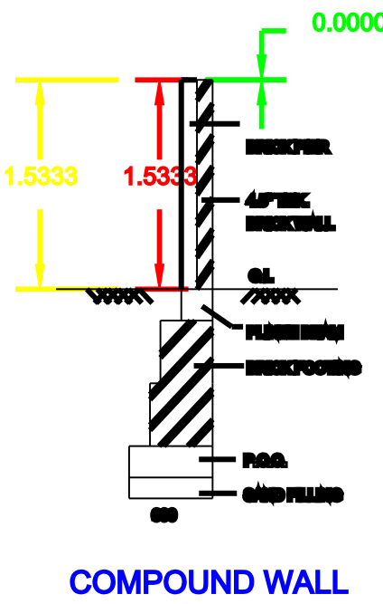
COMPOUND WALL
