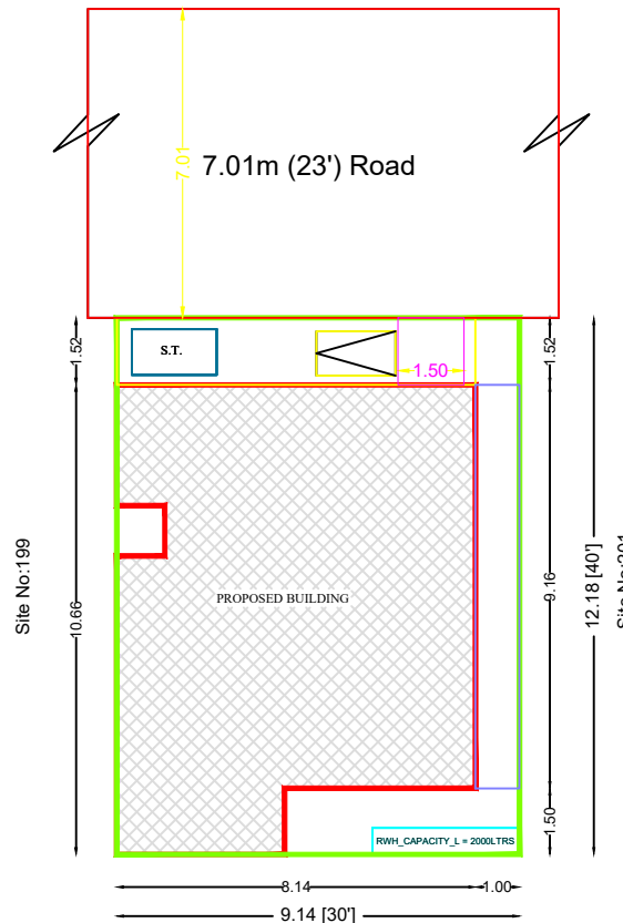
SITE PLAN
