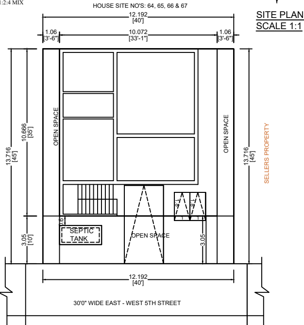
SITE PLAN
