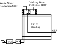
Flow Diagram of Waste Water Recycling & Reuse
