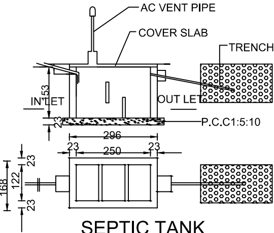
SEPTIC TANK
