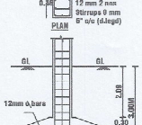
COLUMN DETAILS
