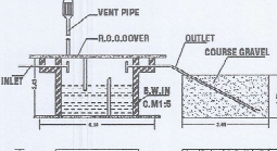
SEPTIC TANK & D-TRENCH DETAILS
