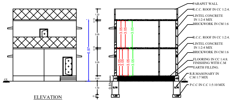
SECTION HK'
