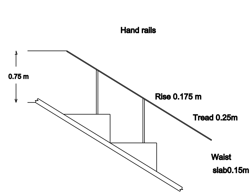
STAIRCASE DETAILS (Not to Scale)
