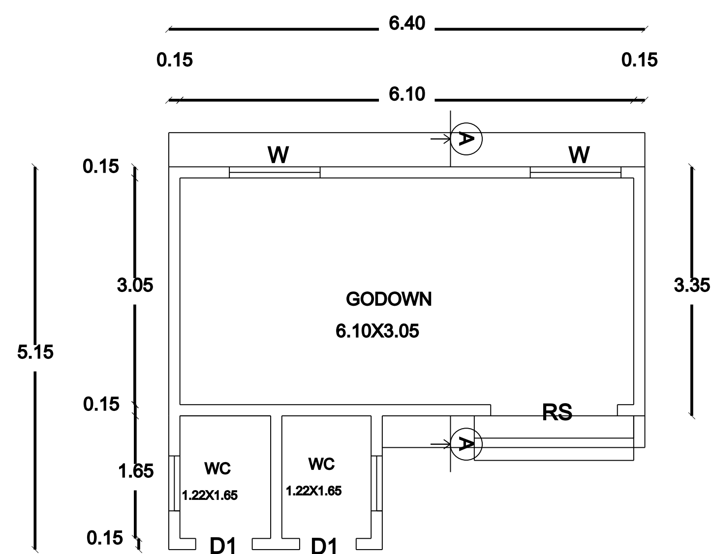
GROUND FLOOR
