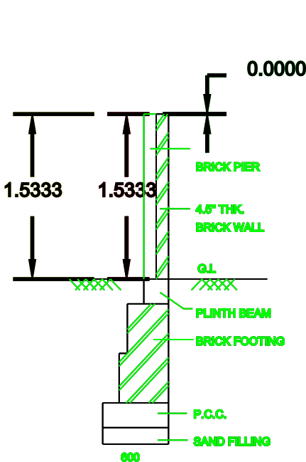
COMPOUND WALL
