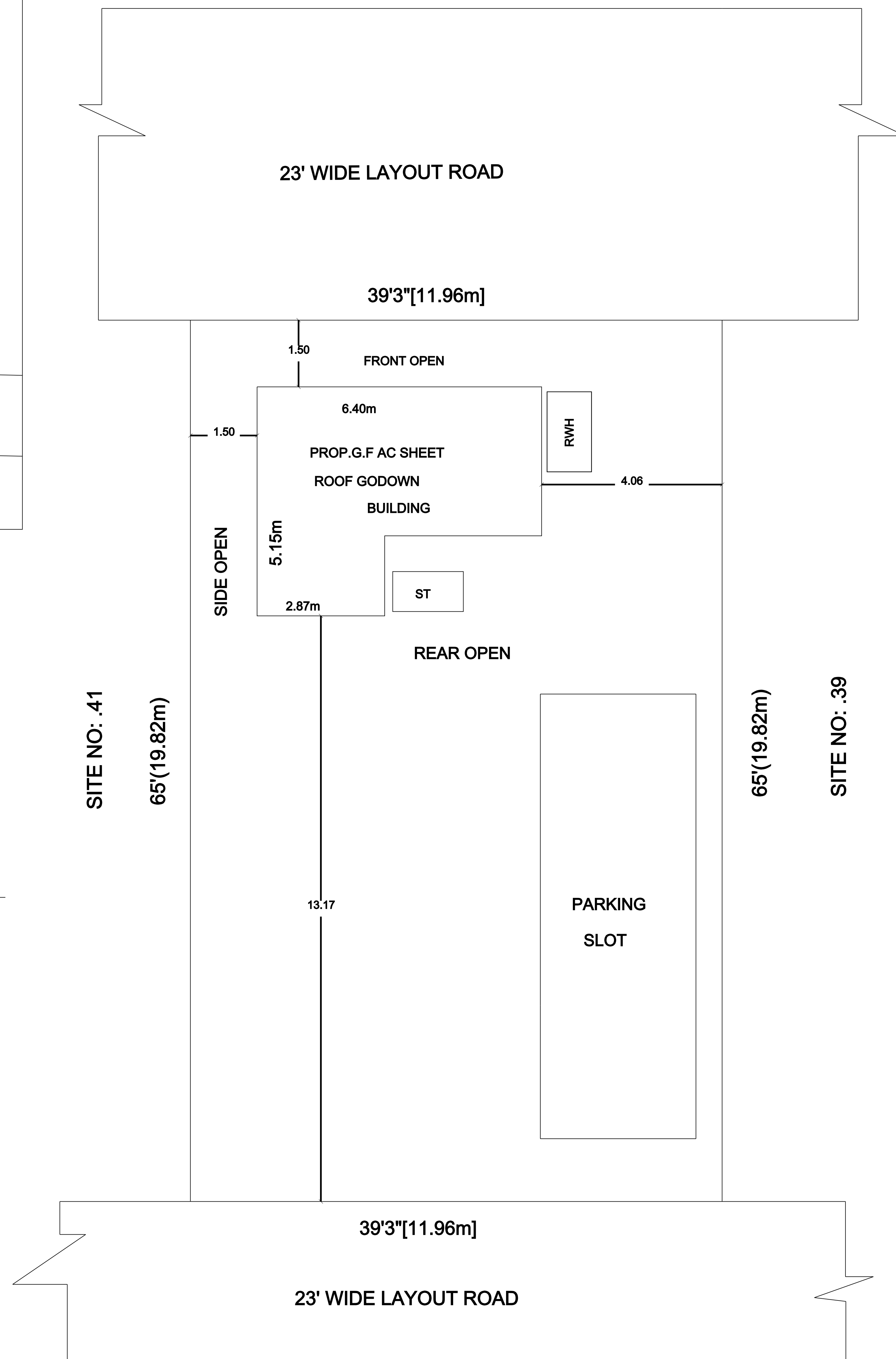
SITE PLAN
