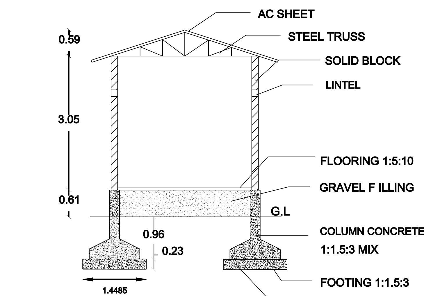
SECTION -AA
