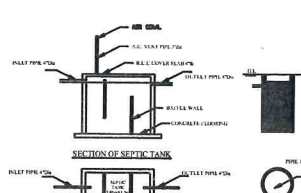
SEPTIC TANK
