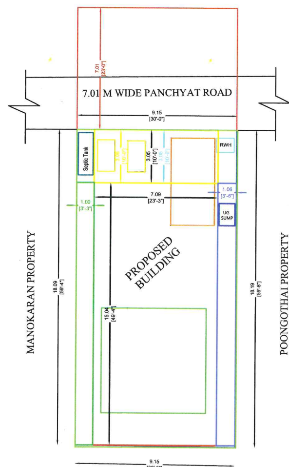
SITE PLAN - (1:100)
