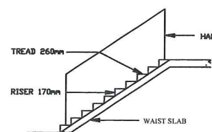
STAIRCASE DETAIL
