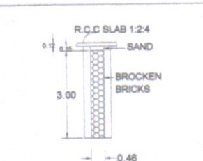
PERCOLATION PIT
