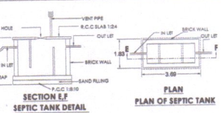
SECTION & PLAN OF SEPTIC TANK
