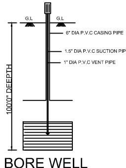
BORE WELL
