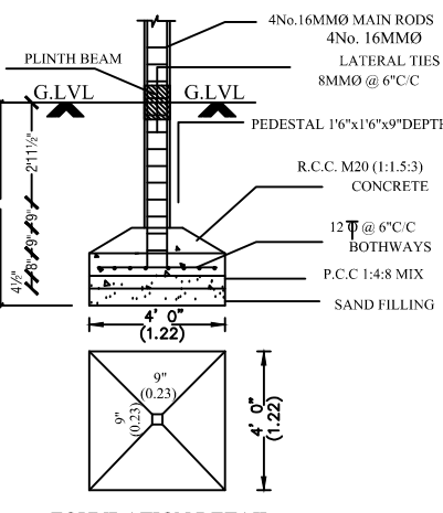
FOUNDATION DETAIL
