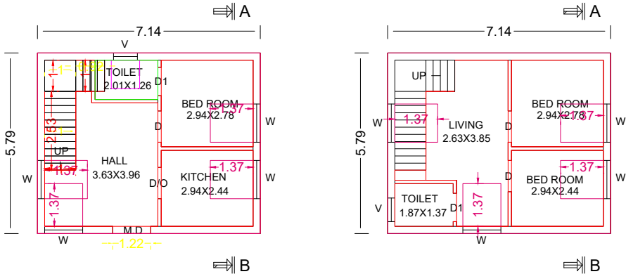
GROUND FLOOR PLAN SCALE 1:100 FLR_HT_M=3.05
