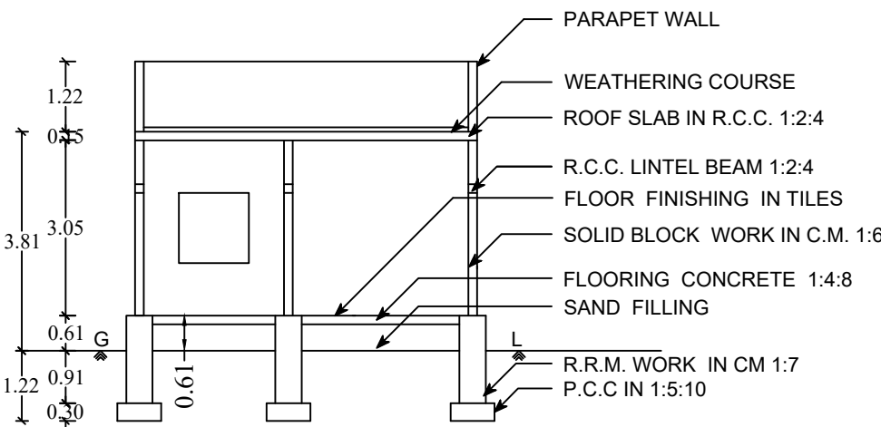
SECTION ON " S S "
