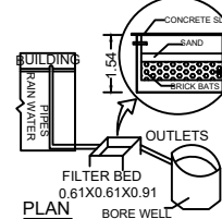
RAIN WATER HARVESTINGSUMP
