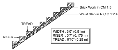
STAIRCASE DETAILS
