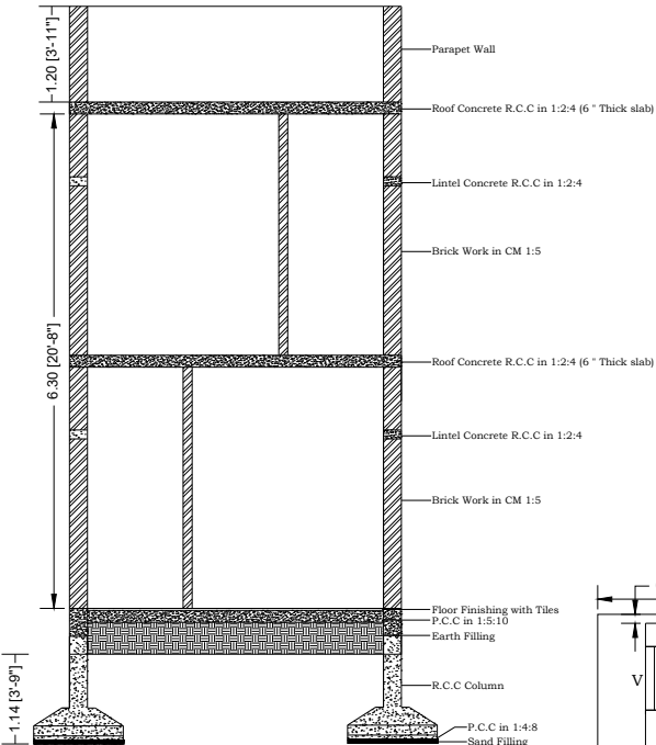
SECTION X-X
