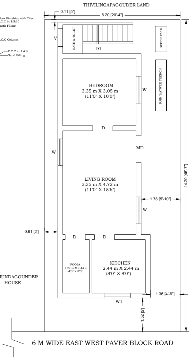
SITE PLAN
