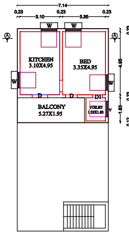
PROPOSED FIRST FLOOR
