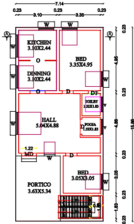
EXISTING GROUND FLOOR
