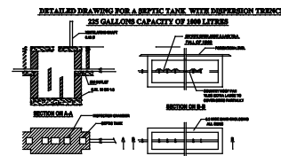
DETAILED DRAWING FOR A RECTANGULAR WATER DISPERSION TRENCH
