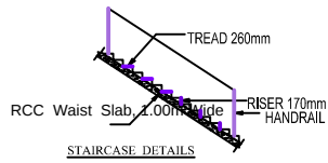
STAIRCASE DETAILS
