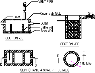
SEPTIC TANK & SOAK PIT DETAILS
