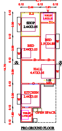
PRO. GROUND FLOOR
