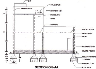
SECTION ON-AA
