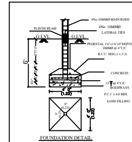
FOUNDATION DETAIL
