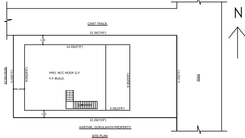
SITE PLAN
