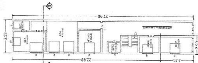
GROUND FLOOR PLAN SCALE 1:100
