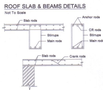
ROOF SLAB & BEAMS DETAILS Not To Scale
