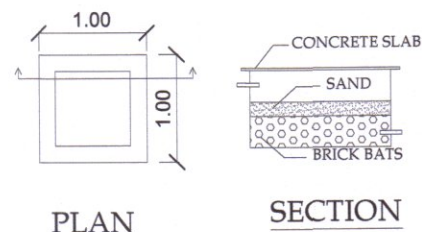
RAIN WATER HARVESTING TANK
