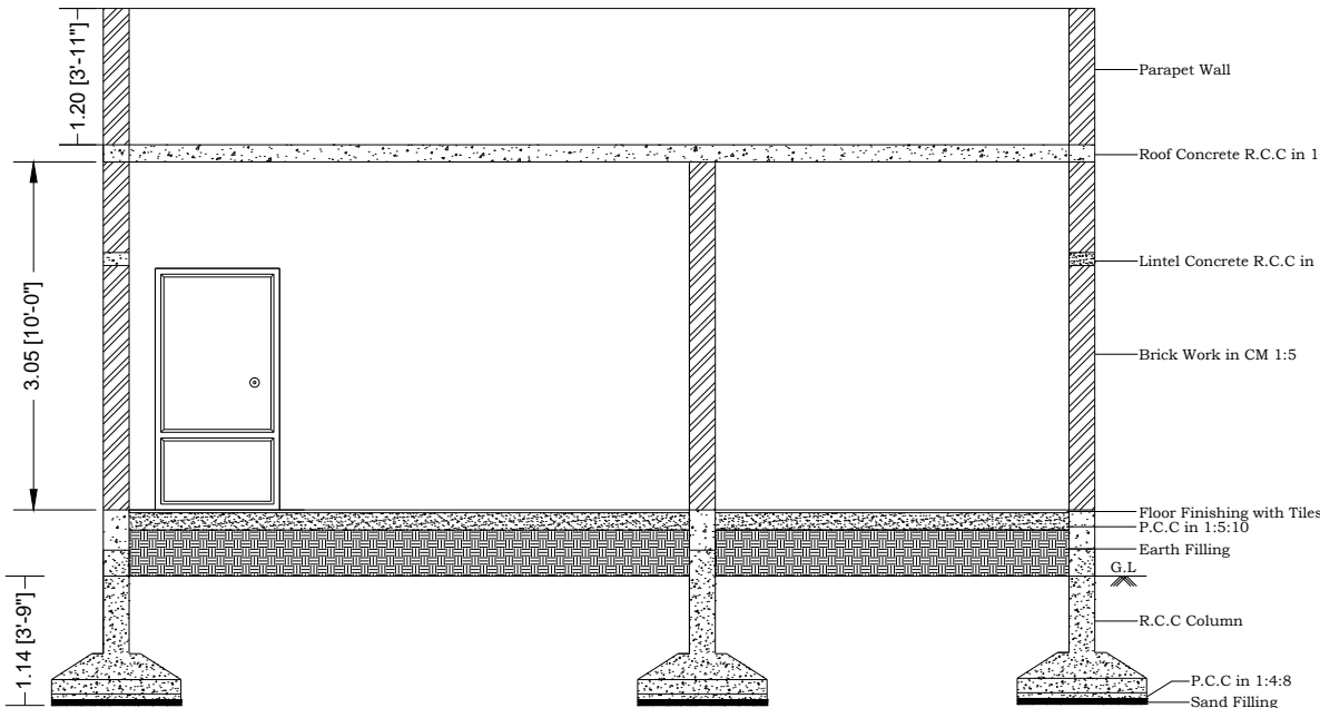
SECTION X-X
