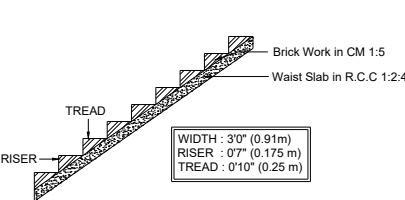
STAIRCASE DETAILS
