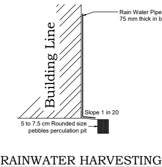
RAINWATER HARVESTING
