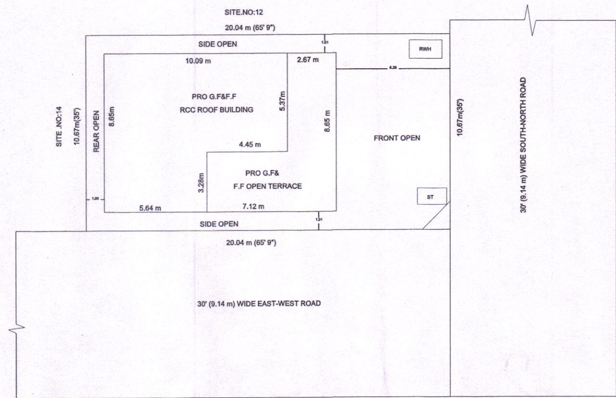
SITE PLAN
