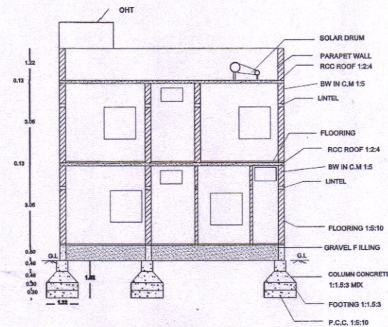
SECTION ON-AA
