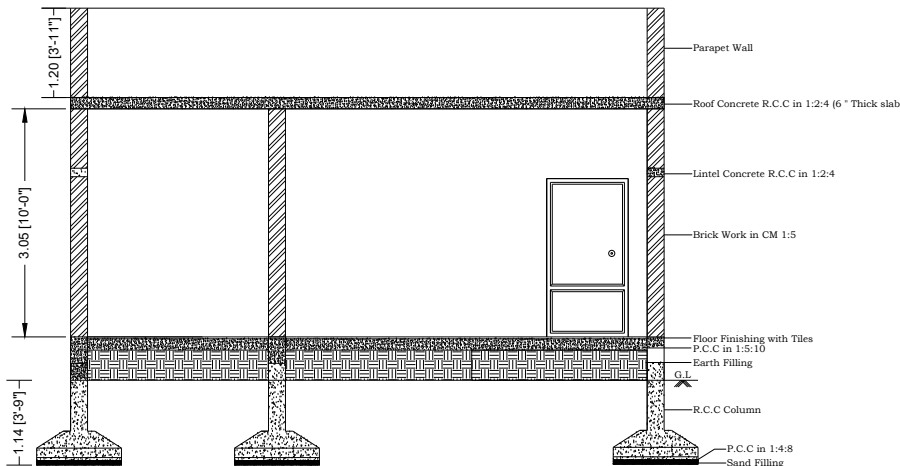
SECTION X-X
