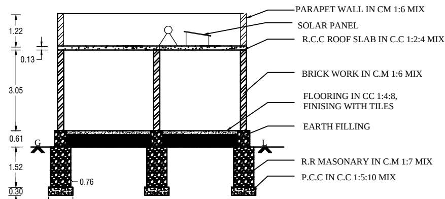
SECTION "A-B"
