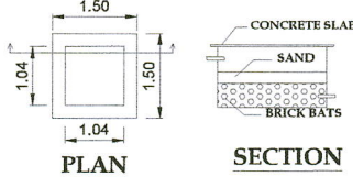
RAIN WATER HARVESTING TANK
