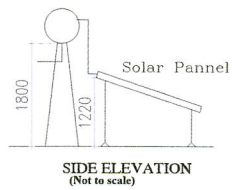
SIDE ELEVATION (Not to scale)
