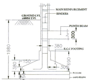
FOUNDATION DETAILS
