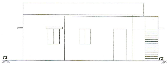
FRONT ELEVATION
