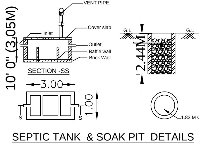
SEPTIC TANK & SOAK PIT DETAILS
