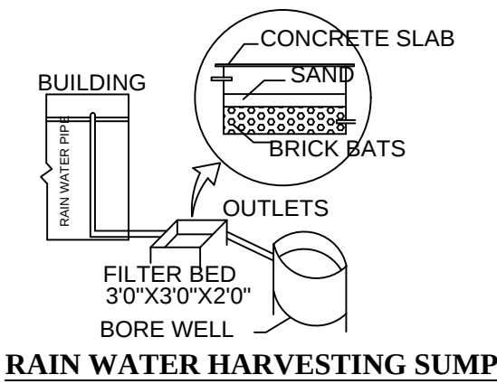
RAIN WATER HARVESTING SUMP
