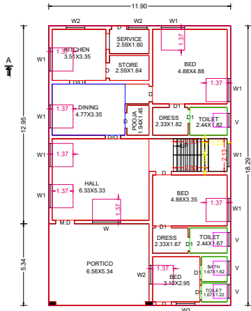
FLR_HT_M=3.05 GROUND FLOOR PLAN SCALE 1:100
