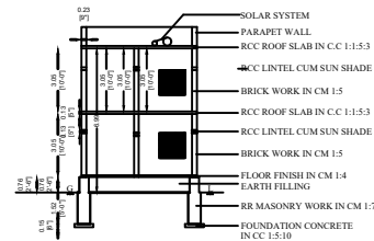
SECTION "AA","BB"
