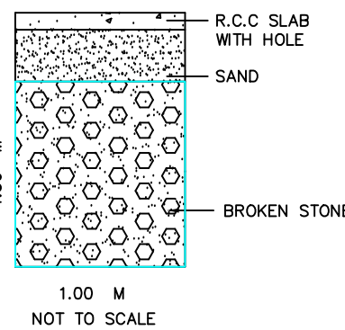
RAIN WATER HARVEST COLLECTION PIT.
