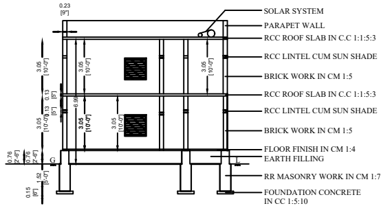
SECTION "AA","BB"
