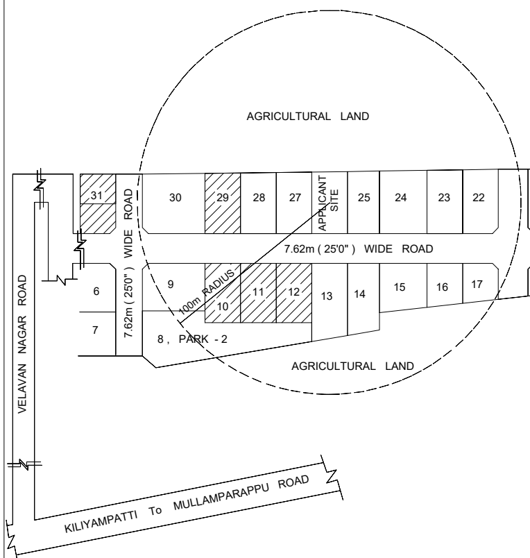
TOPO SKETCH SCALE = 1:1600
