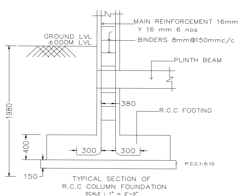
TYPICAL SECTION OF R.C.C COLUMN FOUNDATION SCALE : 1" = 2'-0"
